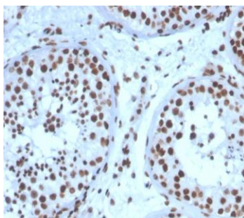
FFPE human testis stained with anti-SF1 using DAB
